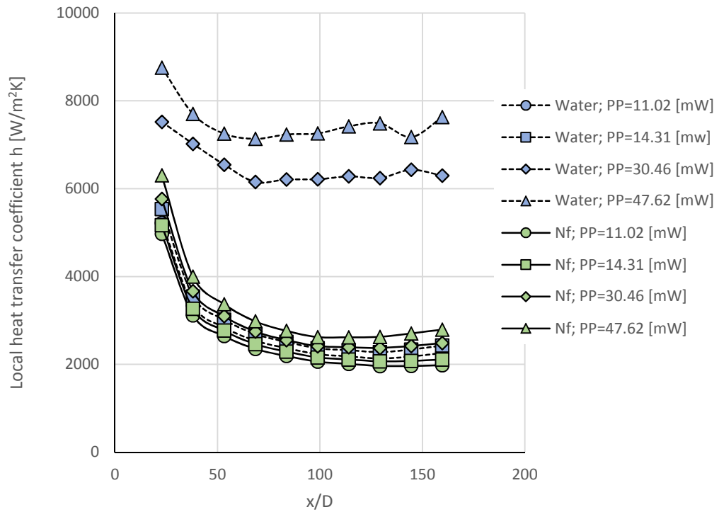
Figure 80. Local heat transfer coefficient h [ \text{W}/\text{m}^2\text{K} ] versus x/d at comparable pumping power 3by32 sq
