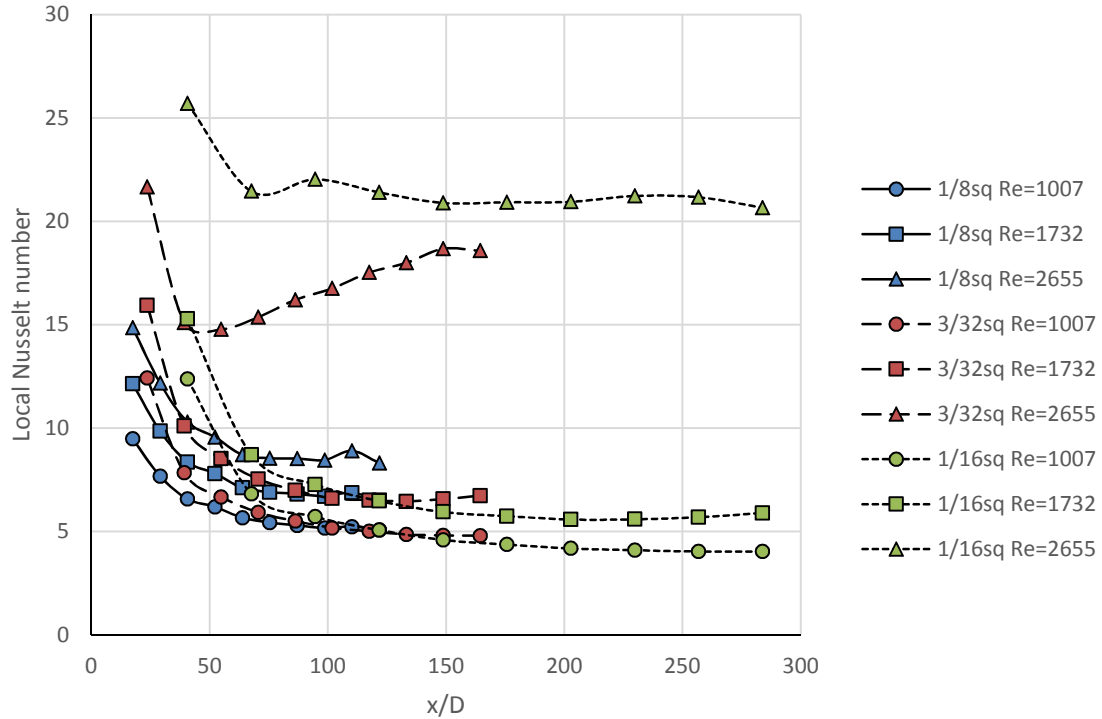
Figure 86. Local Nusselt number versus x/D for \text{SiO}_2 nf in square tubes of different hydraulic diameters
