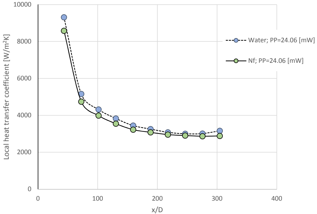
Figure 82. Local heat transfer coefficient h [ W/m^2K ] versus x/D at comparable pumping power in 1by16 sq
