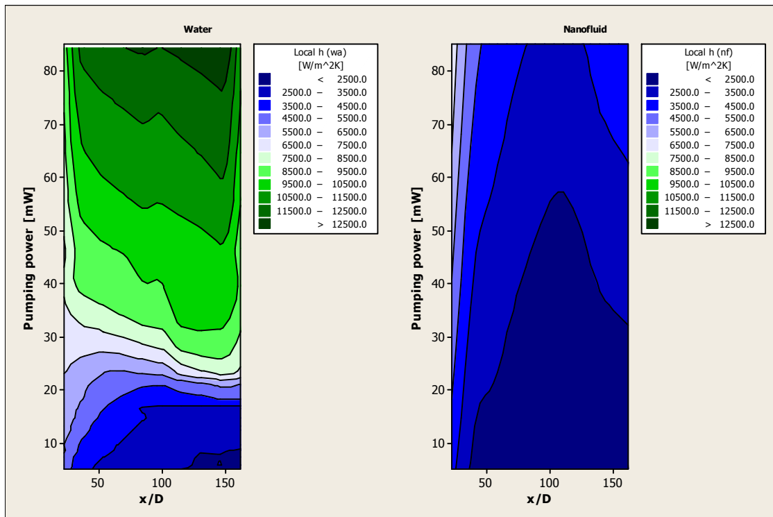
Figure 81. Contour plots for local heat transfer coefficient h [ \text{W}/\text{m}^2\text{K} ] versus pumping power & x/D for water and nf in 3/32sq
