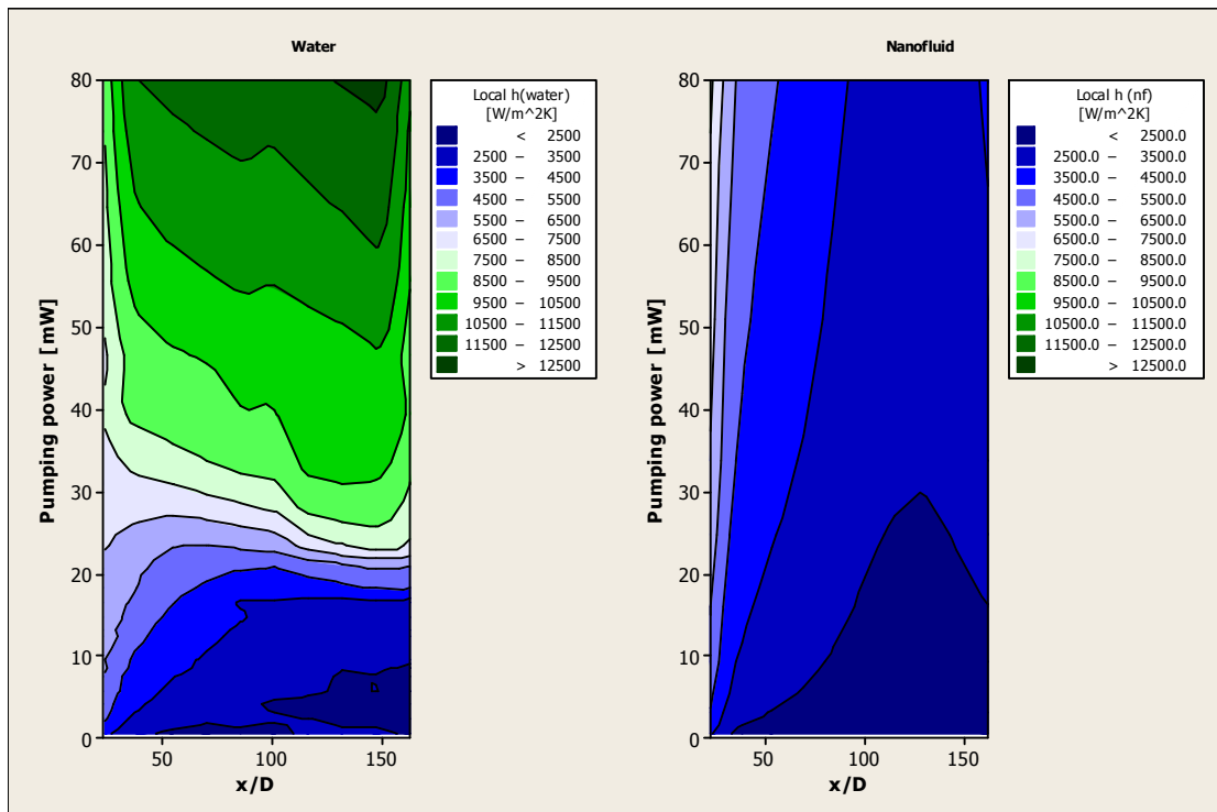
Figure 63. Contour plots for local heat transfer h [ \text{W}/\text{m}^2\text{K} ] versus pumping power [mW] & x/D for water and nf in 3/32c
