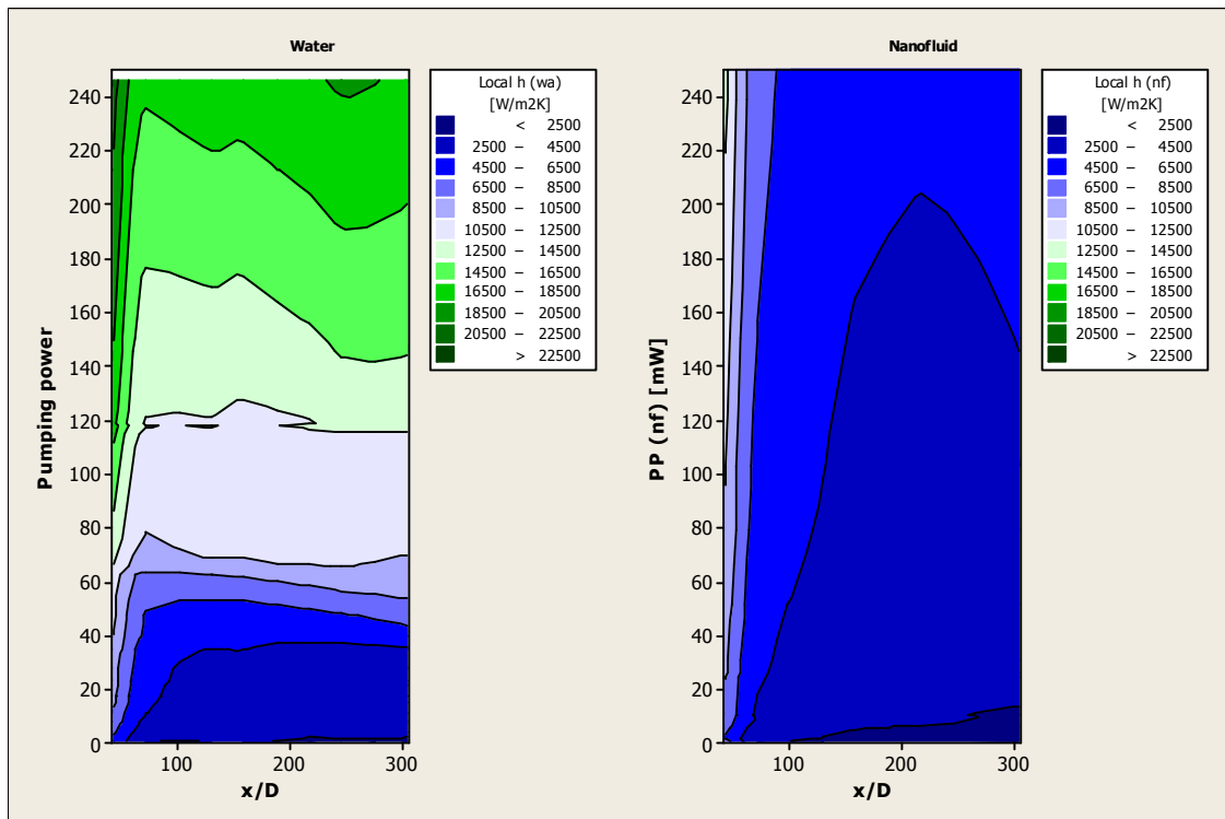
Figure 83. Contour plots for local heattransfer coefficient [ W/m^2K ] h versus pumping power & x/D for water and nf in 1/16sq
