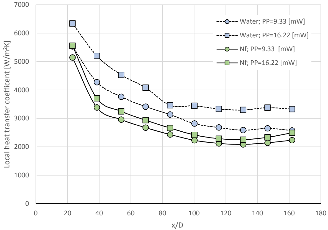
Figure 62. Local heat transfer coefficient h [ \text{W}/\text{m}^2\text{K} ] versus x/D at comparable pumping power [mW] in 3/32c
