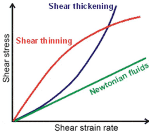
Figure 1. Shear stress-strain plot for Newtonian and non-Newtonian fluids
