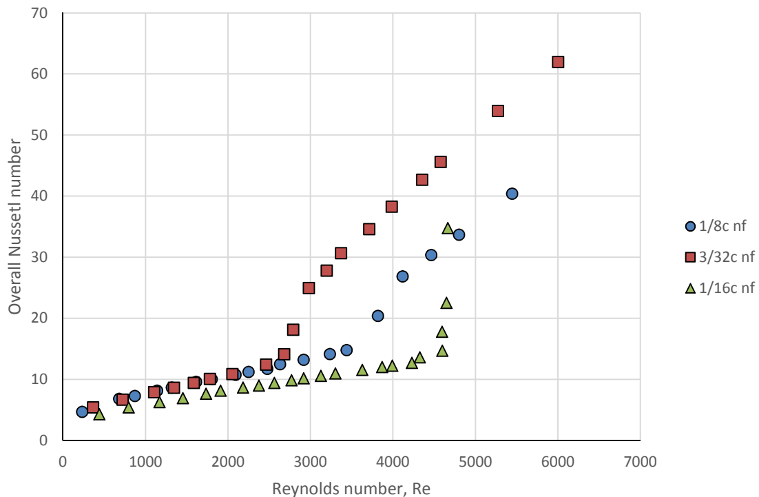
Figure 85. Overall Nusselt number versus Reynolds number for nf in circular tubes of different hydraulic diameters
