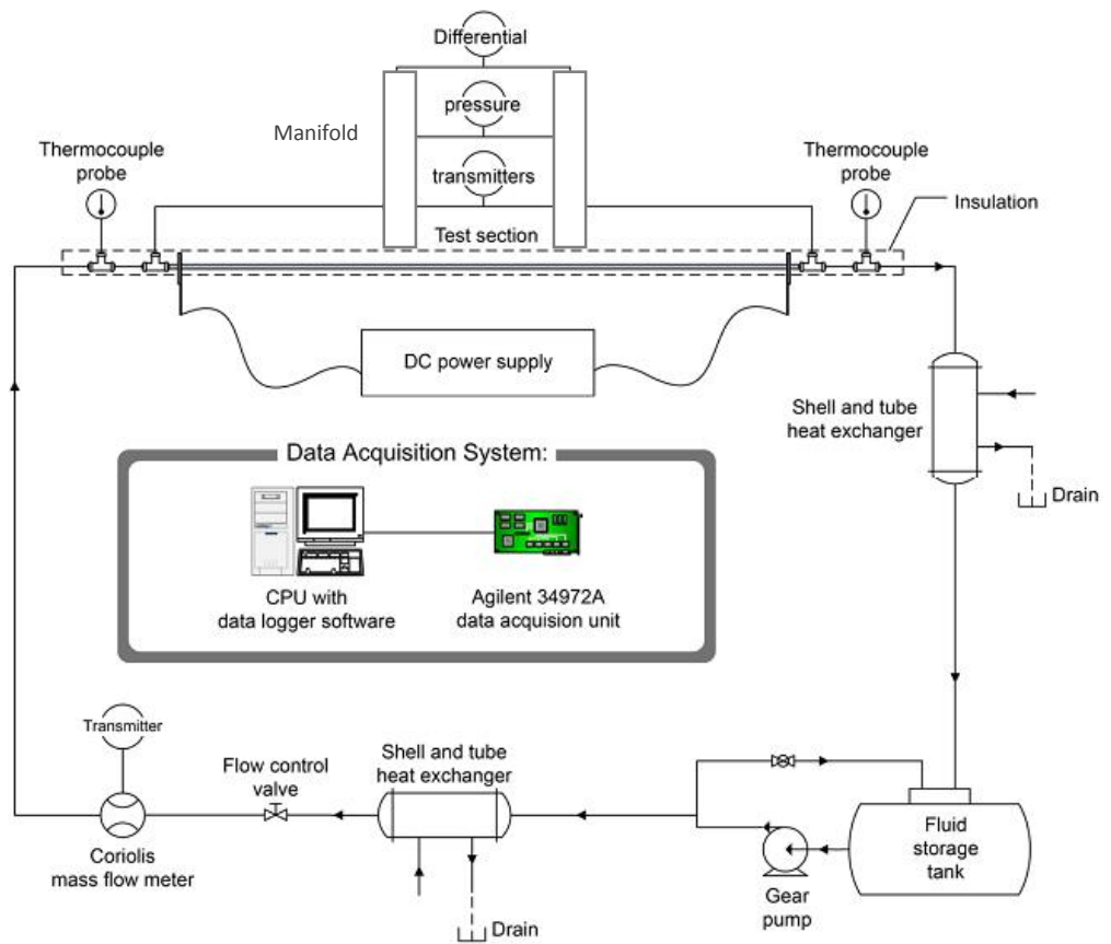
Figure 4. Schematic of the experimental flow loop [8]
